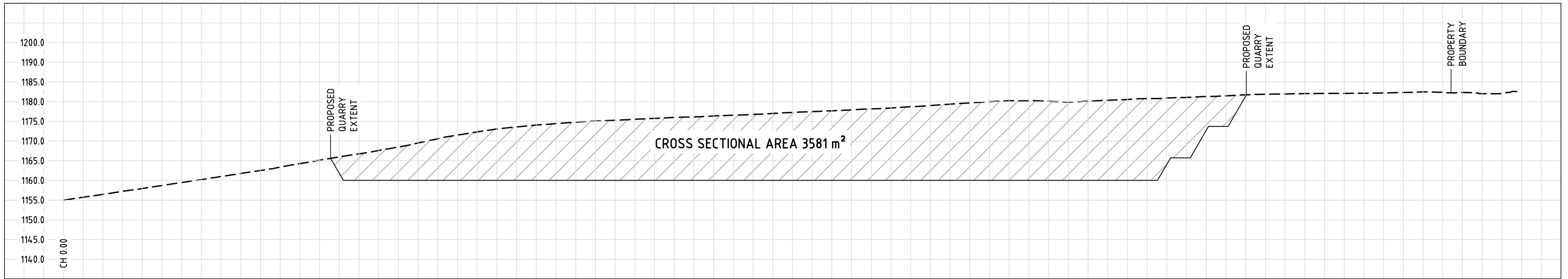
SECTION 02 SCALE 1:500
