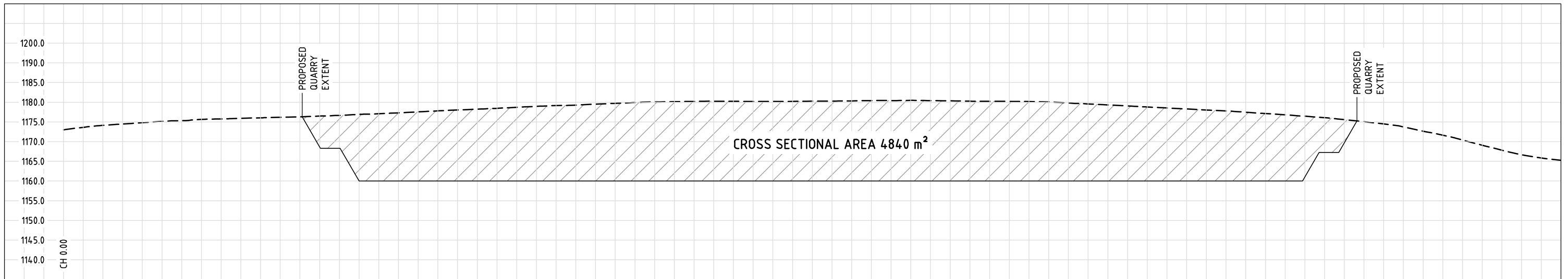
SECTION 03 SCALE 1:500
