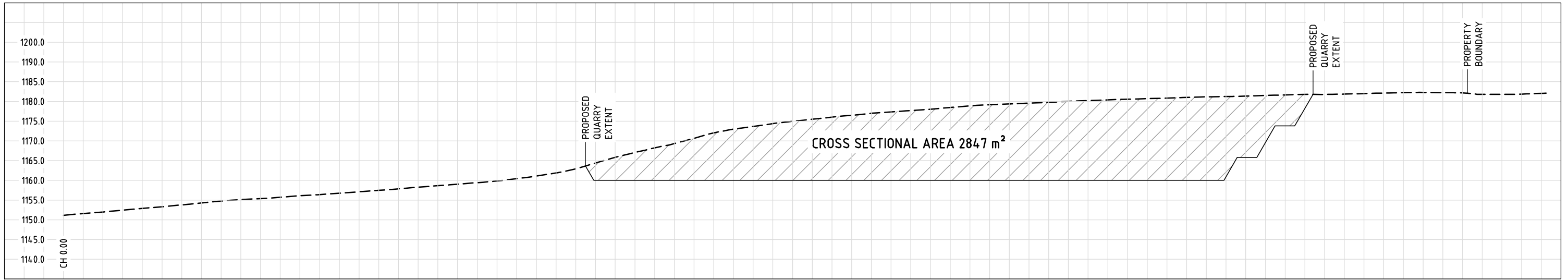
SECTION 01 SCALE 1:500
